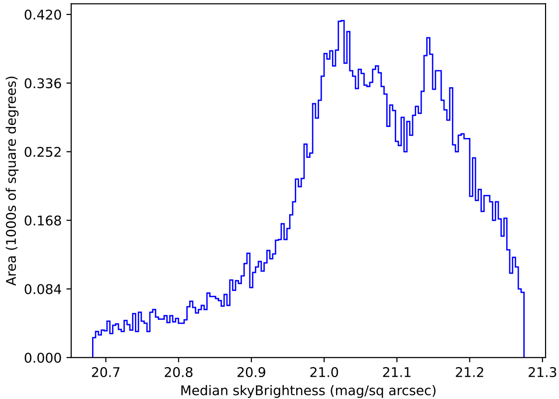
too_elab_2yr_r32_d2_ugrizy_v3.4_10yrs All sky r band: Median skyBrightness
