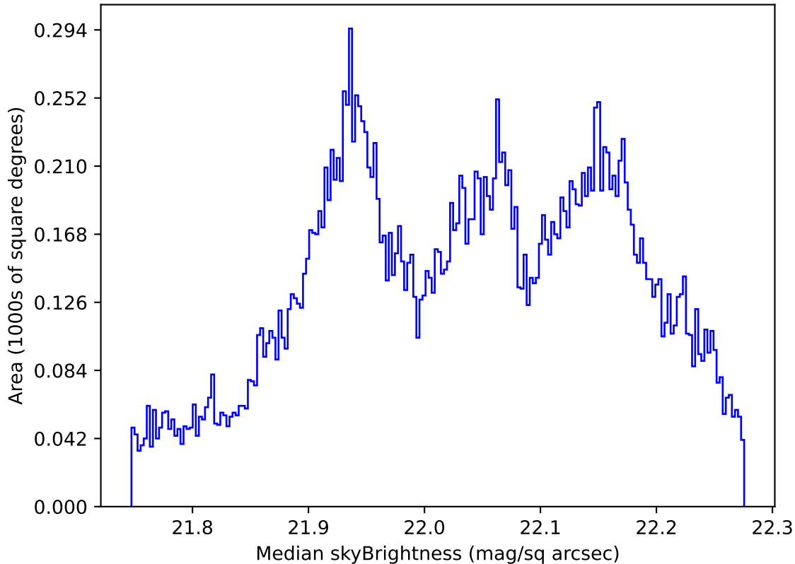
too_elab_2yr_r32_d2_ugrizy_v3.4_10yrs All sky g band: Median skyBrightness
