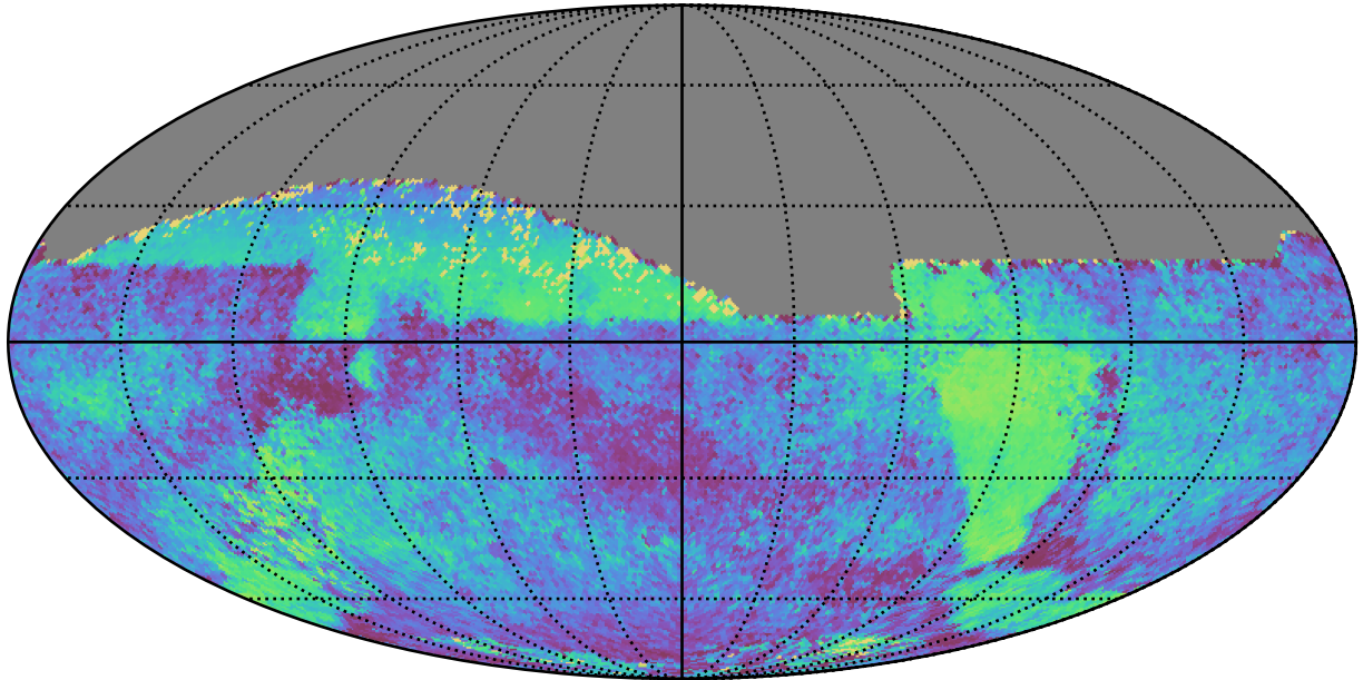
too_elab_2yr_r32_d2_ugrizy_v3.4_10yrs All sky all bands: Median skyBrightness
