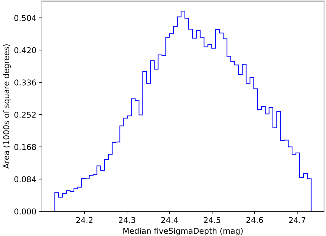
too_elab_2yr_r32_d2_ugrizy_v3.4_10yrs WFD g band: Median fiveSigmaDepth
