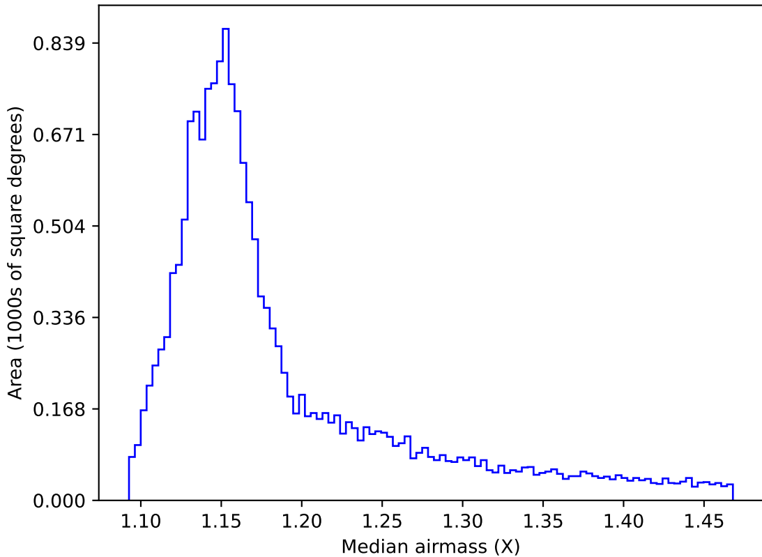
too_elab_2yr_r32_d2_ugrizy_v3.4_10yrs WFD y band: Median airmass
