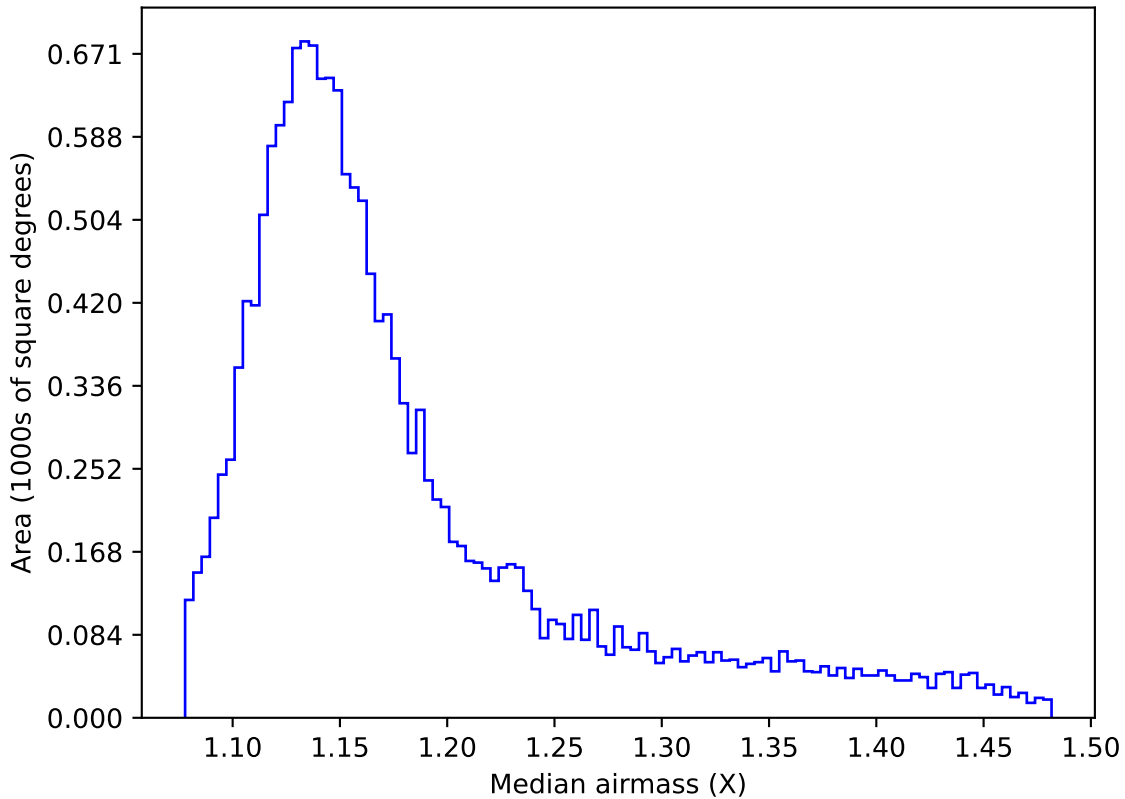
too_elab_2yr_r32_d2_ugrizy_v3.4_10yrs WFD g band: Median airmass
