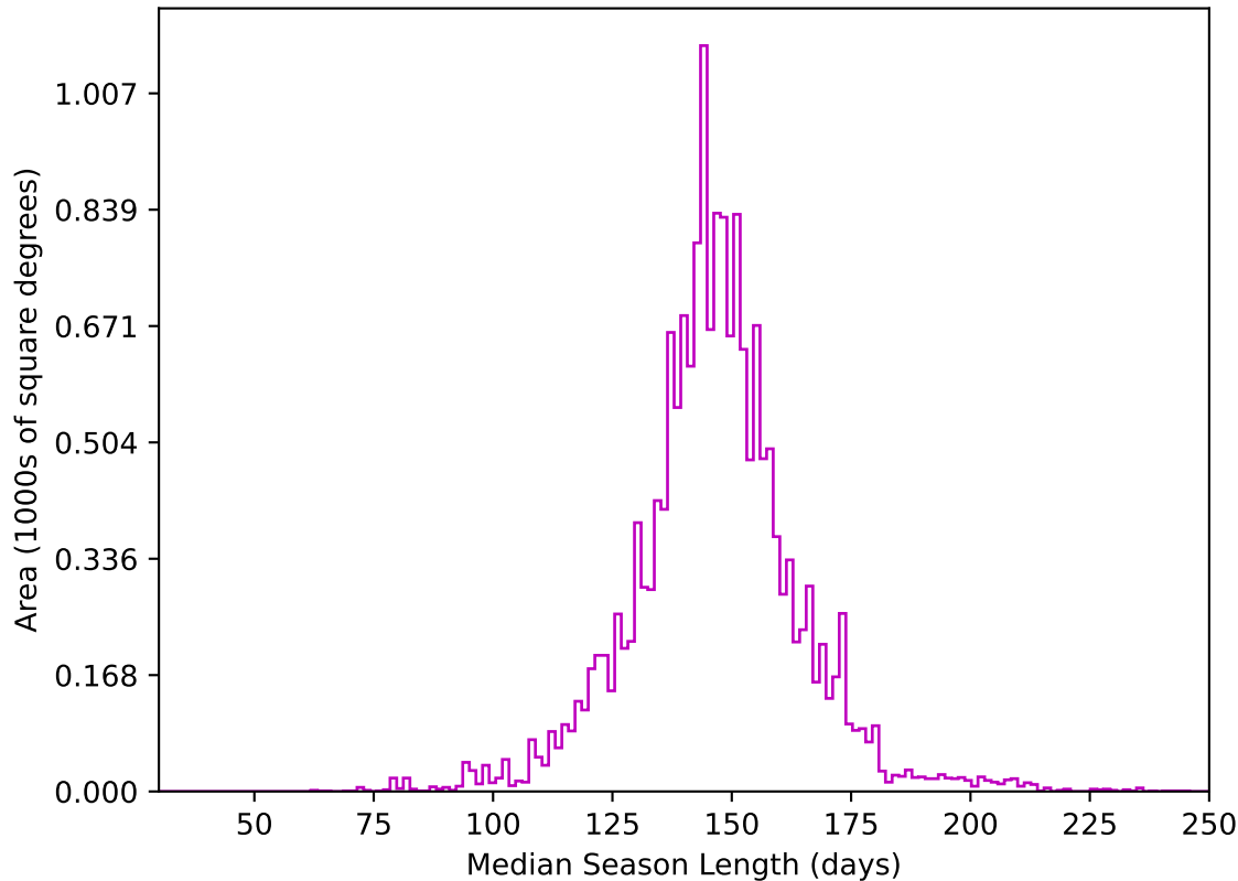
too_elab_2yr_r32_d2_ugrizy_v3.4_10yrs WFD z band: Median Season Length
