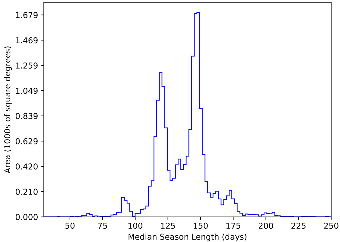
too_elab_2yr_r32_d2_ugrizyv3.4_10yrs WFD y band: Median Season Length
