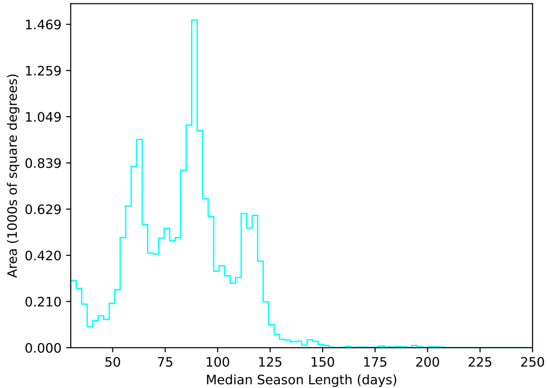
too_elab_2yr_r32_d2_ugrizyv3.4_10yrs WFD u band: Median Season Length
