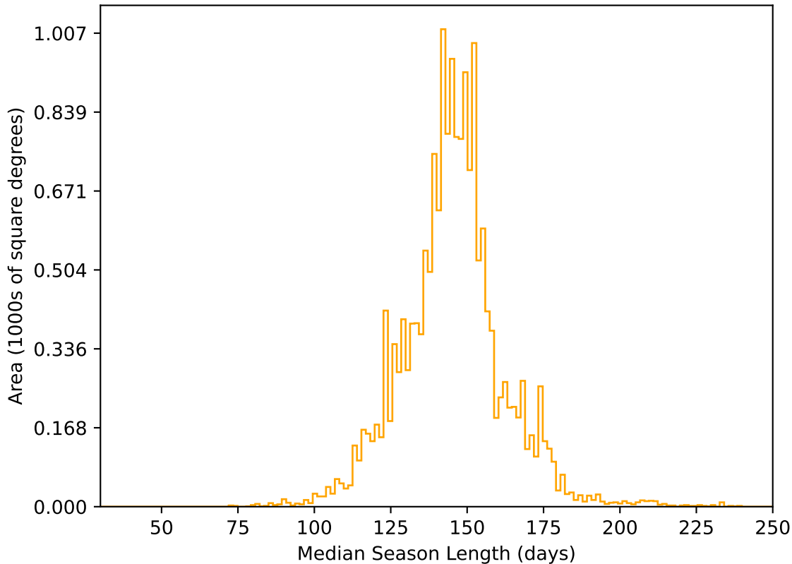
too_elab_2yr_r32_d2_ugrizy_v3.4_10yrs WFD r band: Median Season Length
