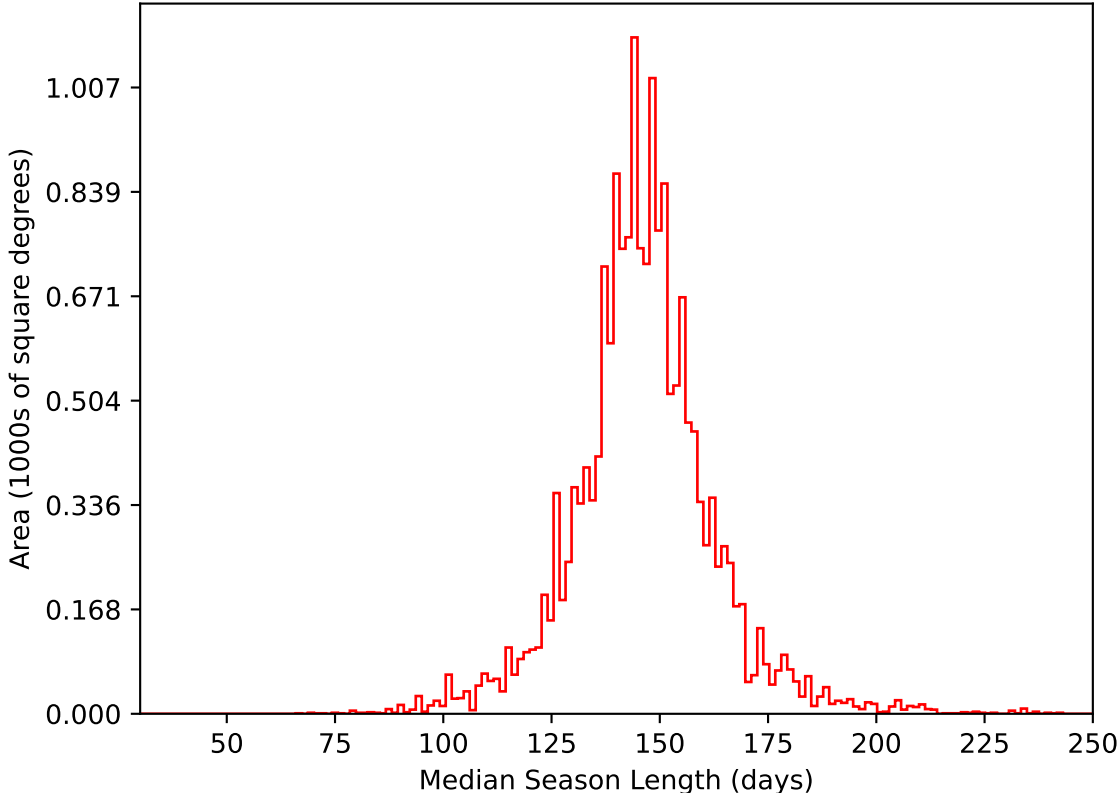
too_elab_2yr_r32_d2_ugrizy_v3.4_10yrs WFD i band: Median Season Length
