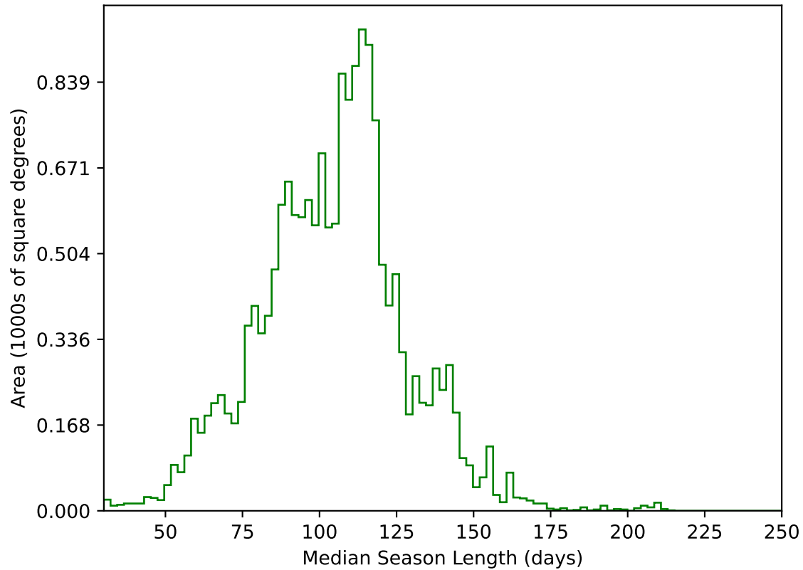
too_elab_2yr_r32_d2_ugrizyv3.4_10yrs WFD g band: Median Season Length
