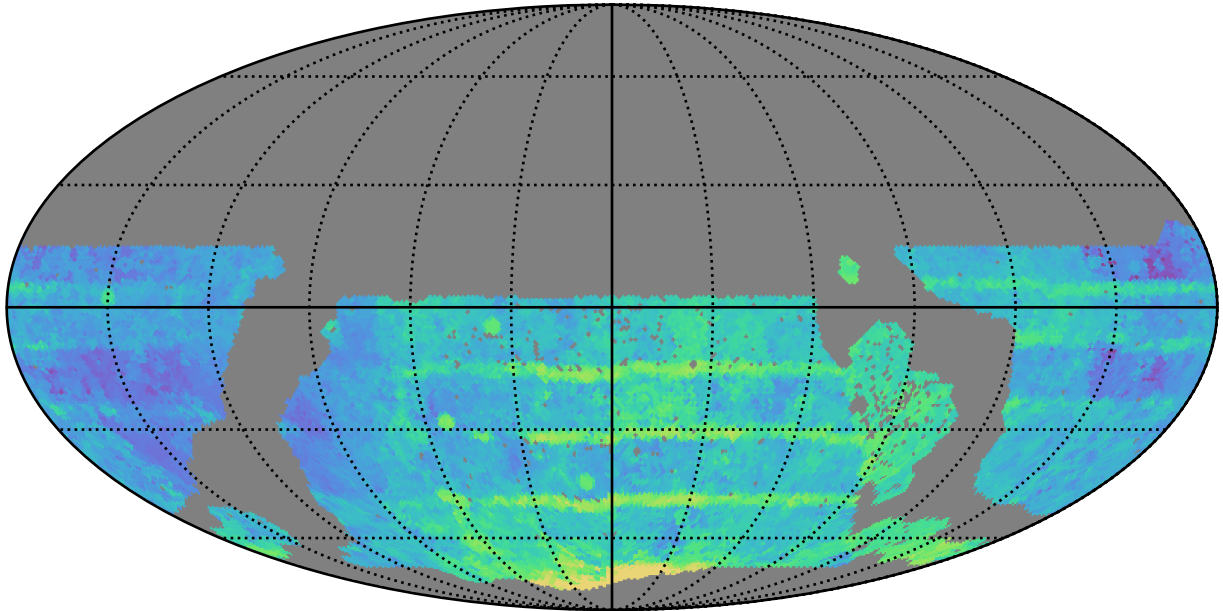
too_elab_2yr_r32_d2_ugrizy_v3.4_10yrs WFD all bands: Median Season Length
