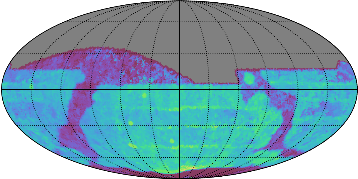
too_elab_2yr_r32_d2_ugrizy_v3.4_10yrs All sky z band: Median Season Length
