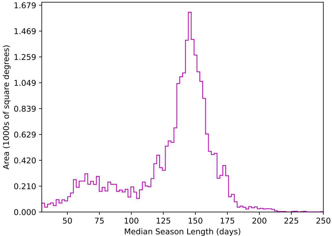
too_elab_2yr_r32_d2_ugrizy_v3.4_10yrs All sky z band: Median Season Length
