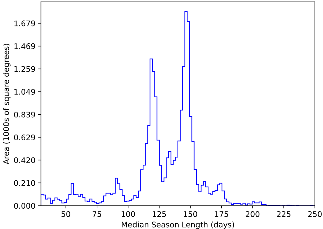
too_elab_2yr_r32_d2_ugrizy_v3.4_10yrs All sky y band: Median Season Length
