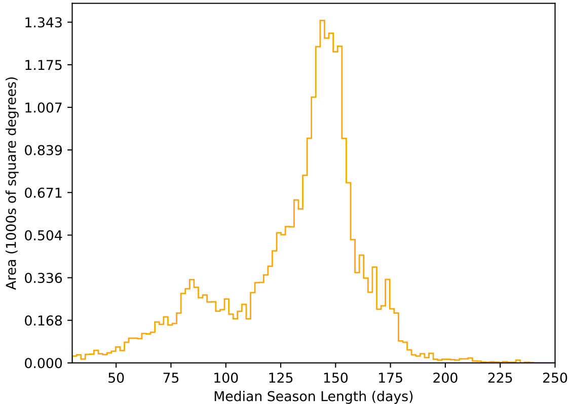
too_elab_2yr_r32_d2_ugrizy_v3.4_10yrs All sky r band: Median Season Length
