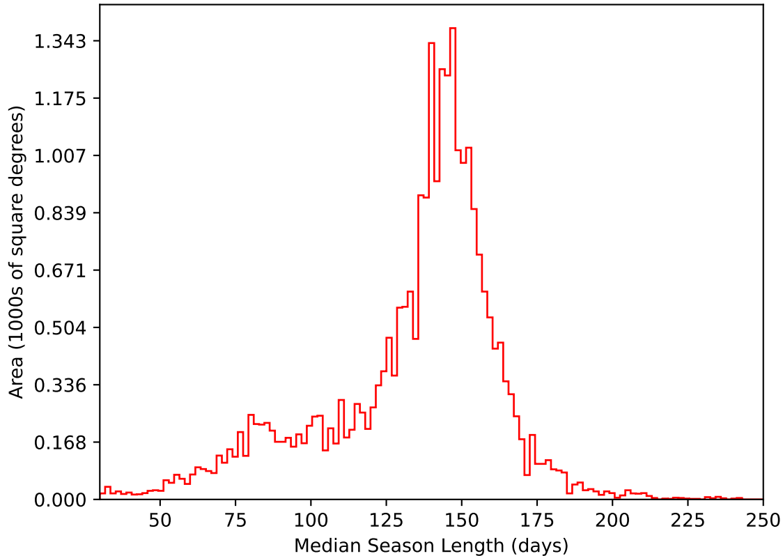
too_elab_2yr_r32_d2_ugrizy_v3.4_10yrs All sky i band: Median Season Length
