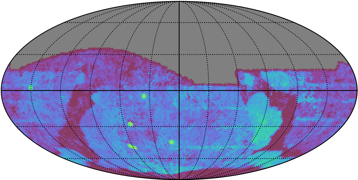
too_elab_2yr_r32_d2_ugrizy_v3.4_10yrs All sky g band: Median Season Length
