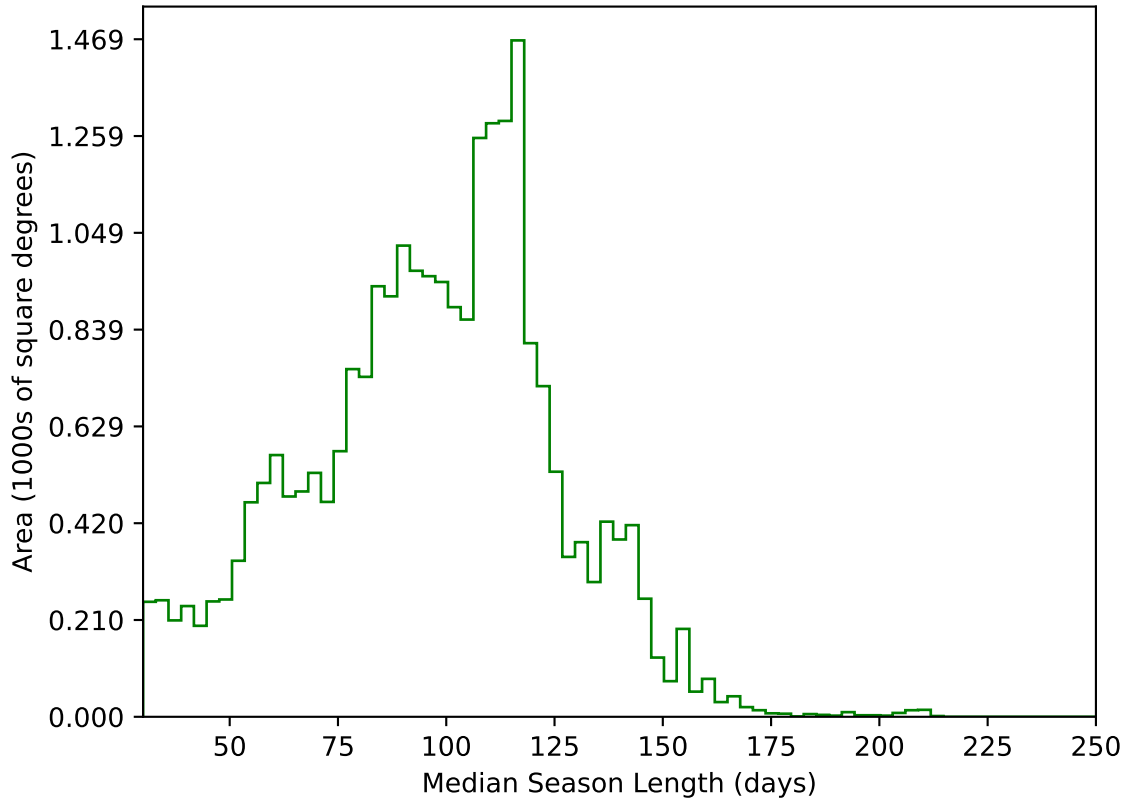
too_elab_2yr_r32_d2_ugrizy_v3.4_10yrs All sky g band: Median Season Length
