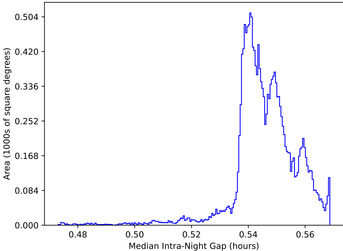
too_elab_2yr_r32_d2_ugrizy_v3.4_10yrs WFD: Median Intra-Night Gap
