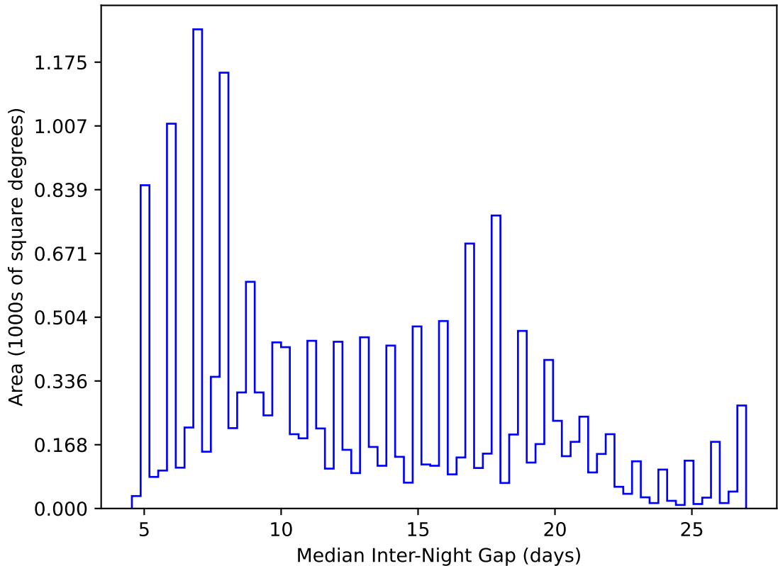
too_elab_2yr_r32_d2_ugrizy_v3.4_10yrs WFD y band: Median Inter-Night Gap
