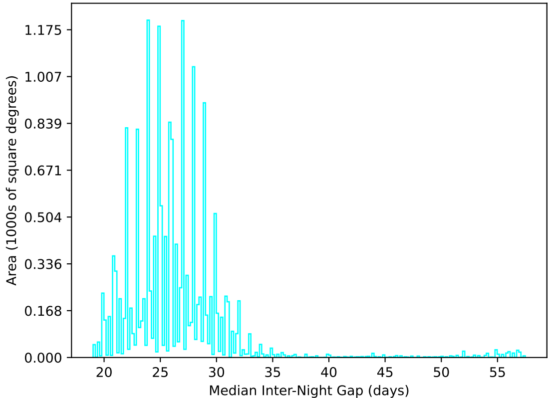
too_elab_2yr_r32_d2_ugrizyv3.4_10yrs WFD u band: Median Inter-Night Gap
