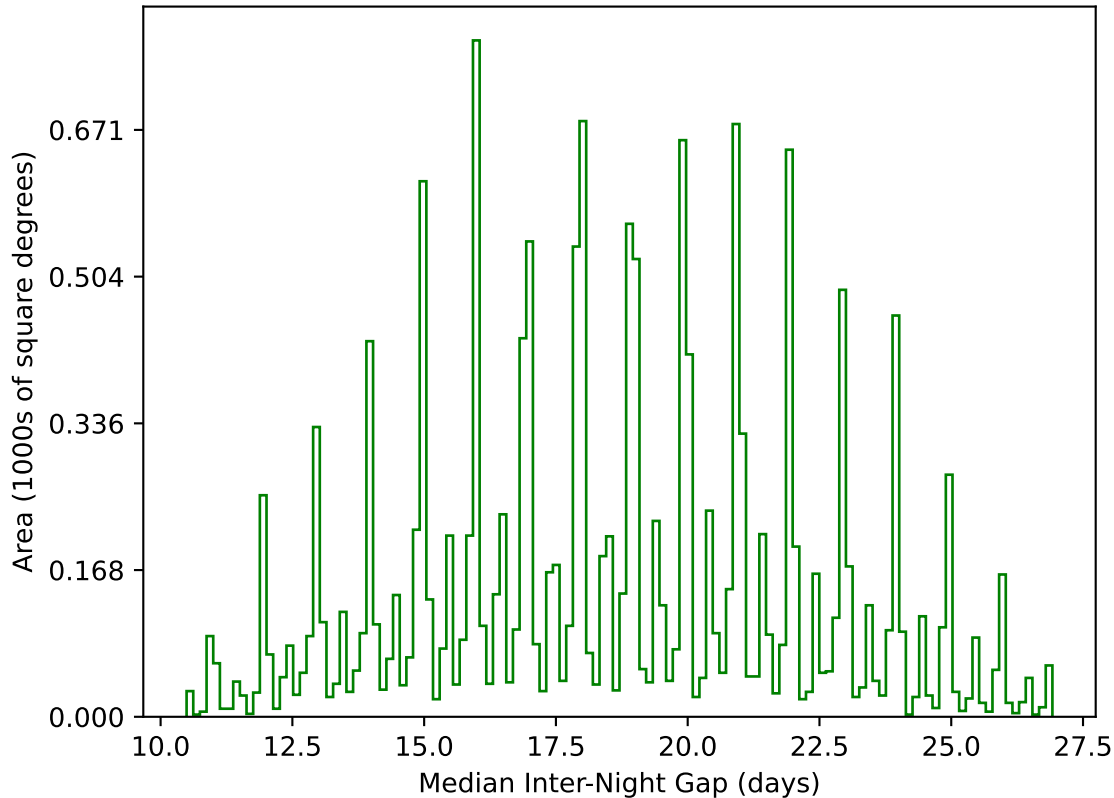
too_elab_2yr_r32_d2_ugrizy_v3.4_10yrs WFD g band: Median Inter-Night Gap
