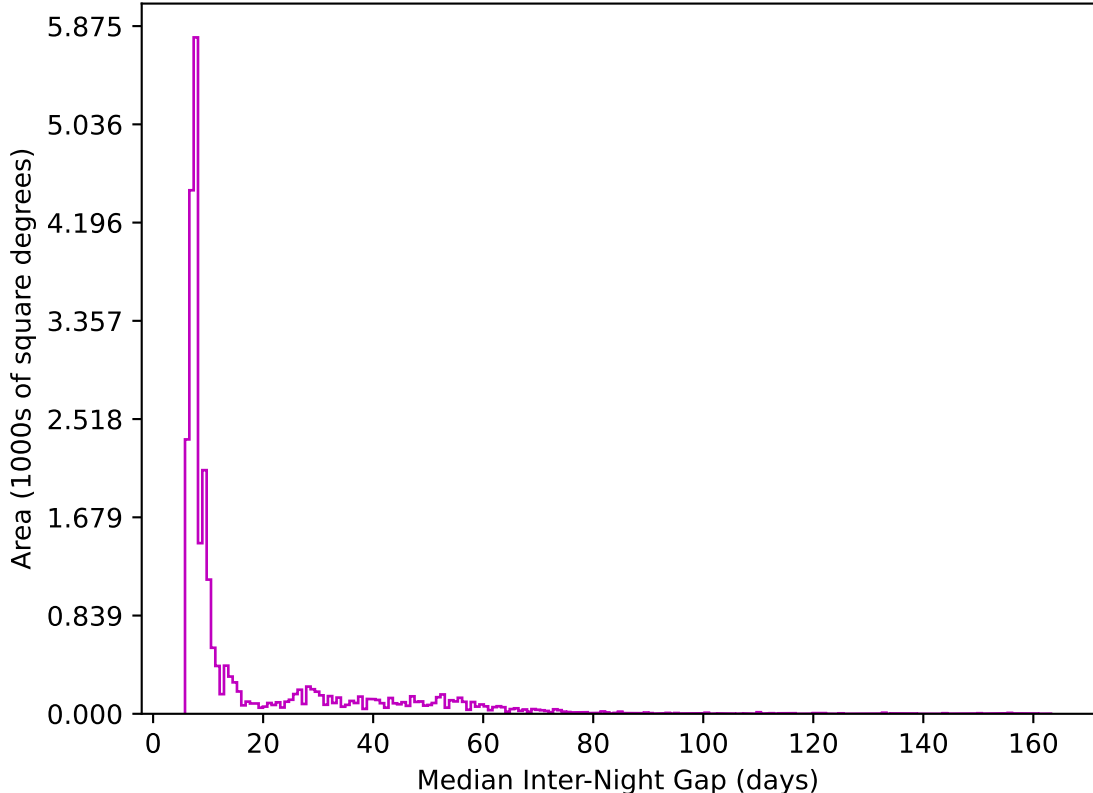
too_elab_2yr_r32_d2_ugrizy_v3.4_10yrs All sky z band: Median Inter-Night Gap
