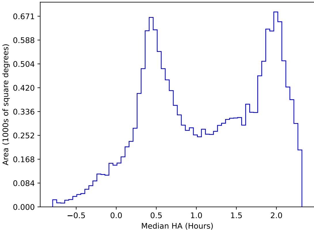
too_elab_2yr_r32_d2_ugrizy_v3.4_10yrs WFD z band: Median HA
