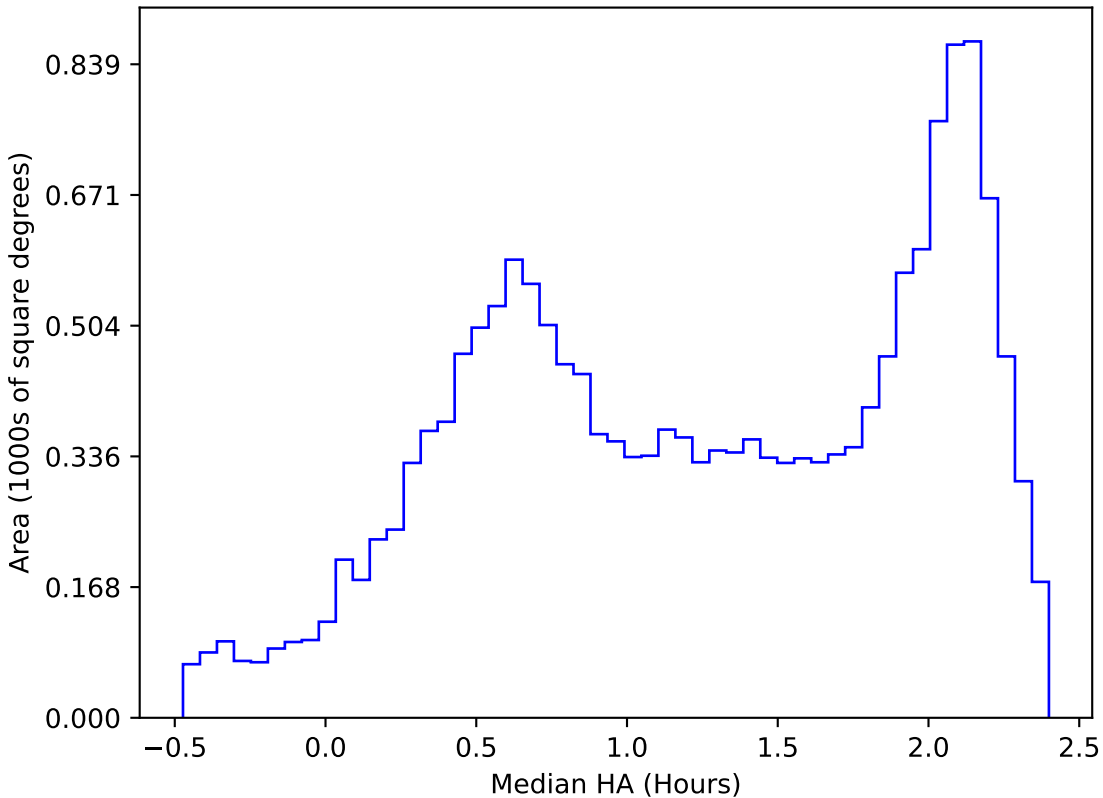
too_elab_2yr_r32_d2_ugrizy_v3.4_10yrs WFD y band: Median HA
