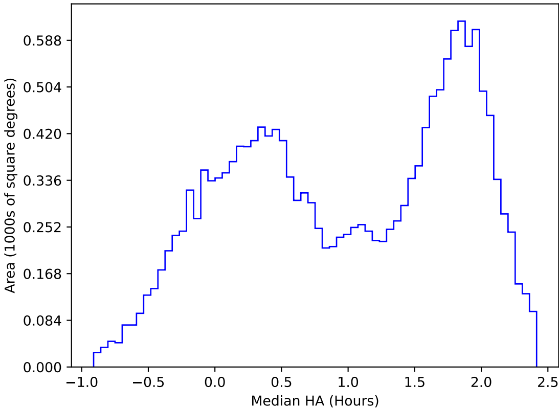
too_elab_2yr_r32_d2_ugrizy_v3.4_10yrs WFD u band: Median HA
