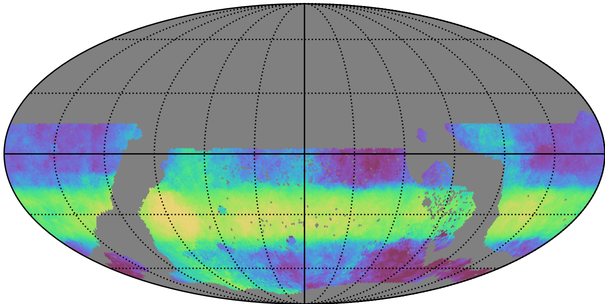
too_elab_2yr_r32_d2_ugrizy_v3.4_10yrs WFD r band: Median HA
