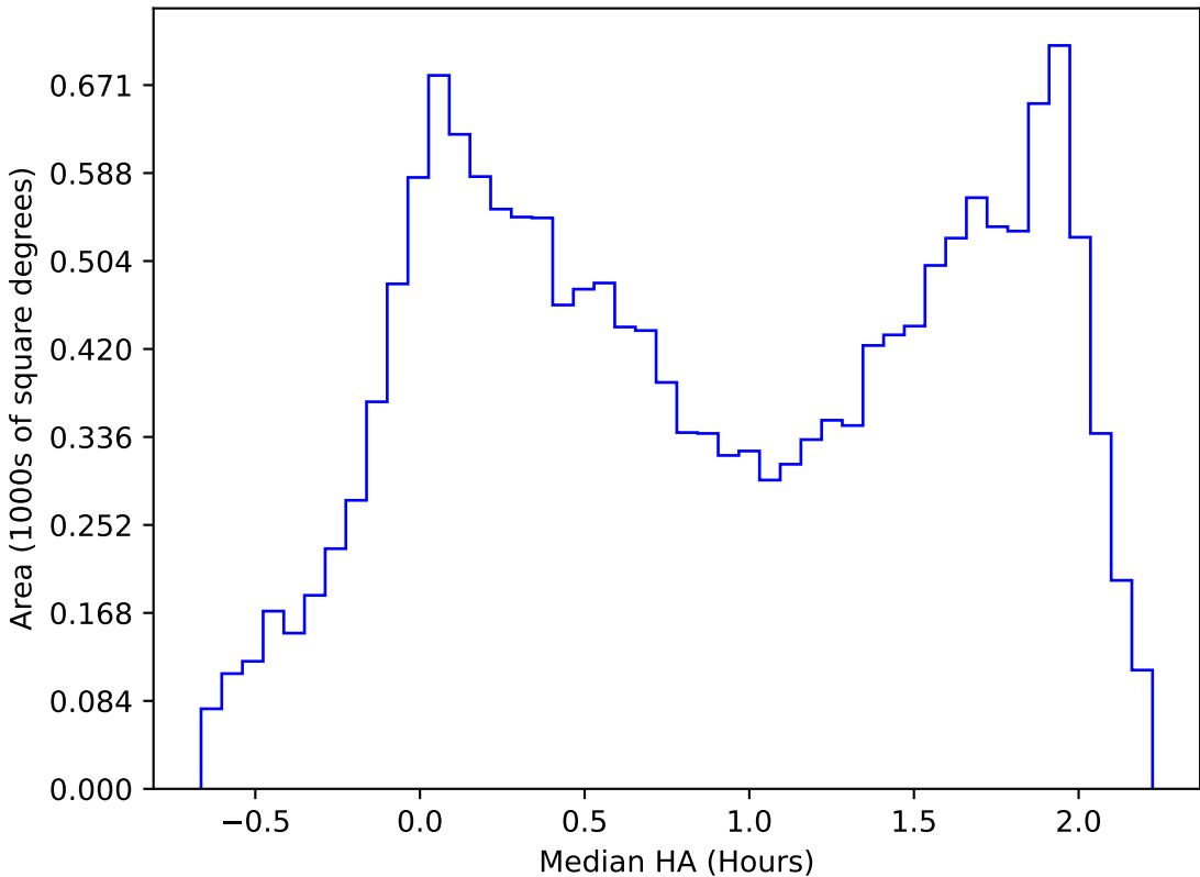
too_elab_2yr_r32_d2_ugrizy_v3.4_10yrs WFD r band: Median HA
