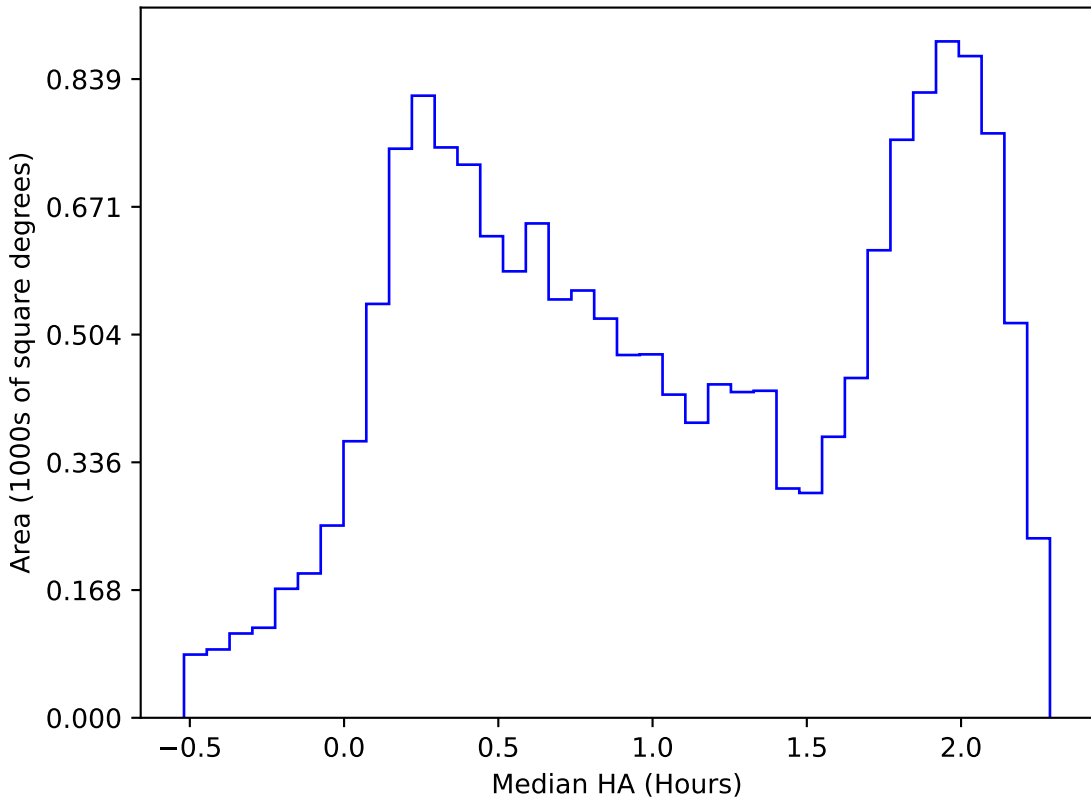
too_elab_2yr_r32_d2_ugrizy_v3.4_10yrs WFD i band: Median HA
