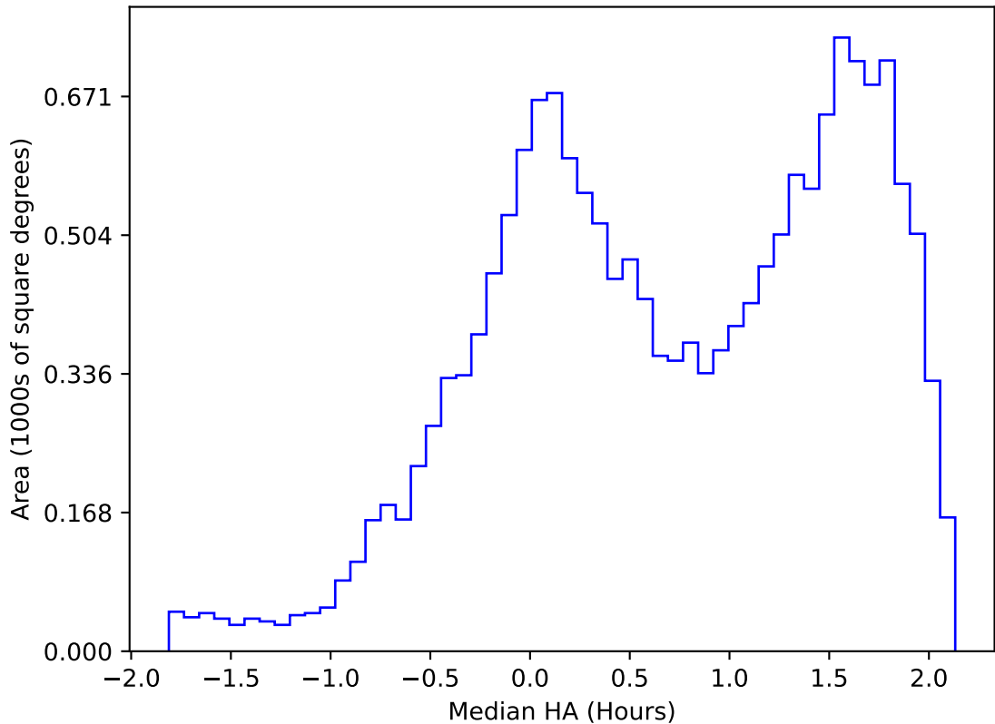
too_elab_2yr_r32_d2_ugrizy_v3.4_10yrs WFD g band: Median HA
