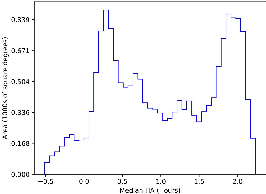
too_elab_2yr_r32_d2_ugrizy_v3.4_10yrs WFD all bands: Median HA
