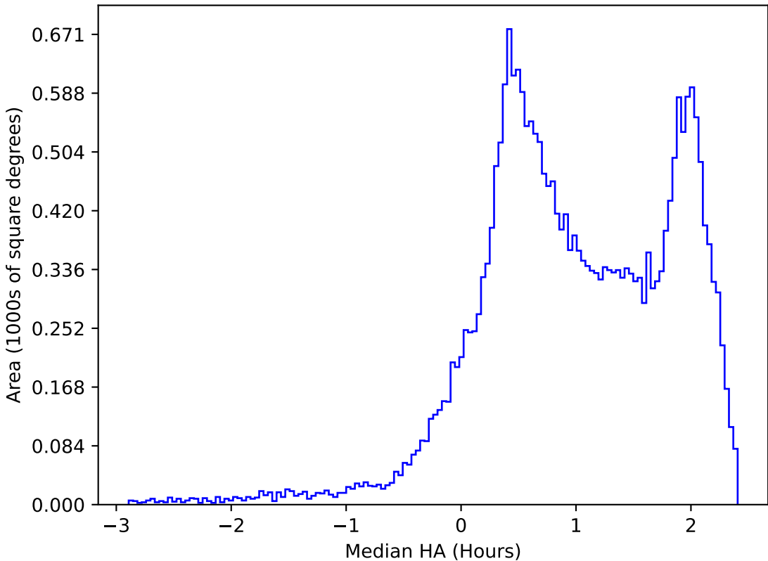
too_elab_2yr_r32_d2_ugrizy_v3.4_10yrs All sky z band: Median HA
