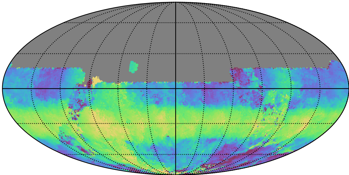
too_elab_2yr_r32_d2_ugrizy_v3.4_10yrs All sky u band: Median HA
