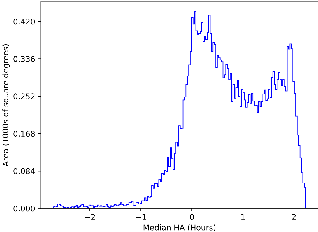
too_elab_2yr_r32_d2_ugrizy_v3.4_10yrs All sky r band: Median HA
