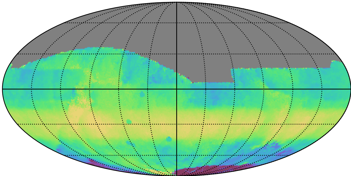
too_elab_2yr_r32_d2_ugrizy_v3.4_10yrs All sky i band: Median HA
