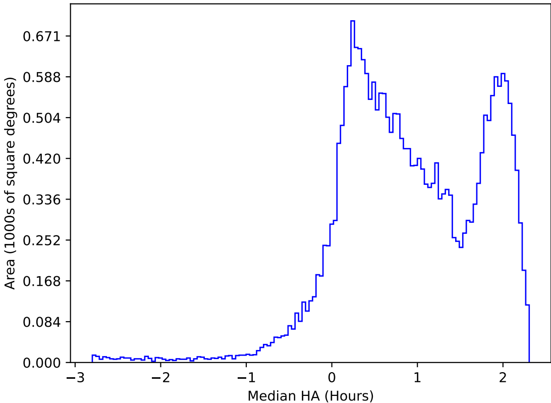
too_elab_2yr_r32_d2_ugrizy_v3.4_10yrs All sky i band: Median HA
