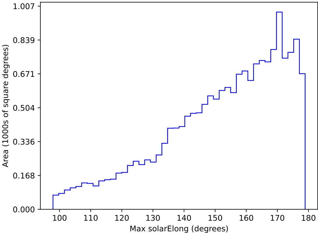
too_elab_2yr_r32_d2_ugrizy_v3.4_10yrs WFD u band: Max solarElong
