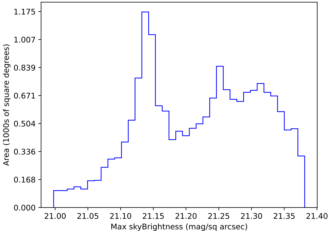
too_elab_2yr_r32_d2_ugrizy_v3.4_10yrs WFD r band: Max skyBrightness
