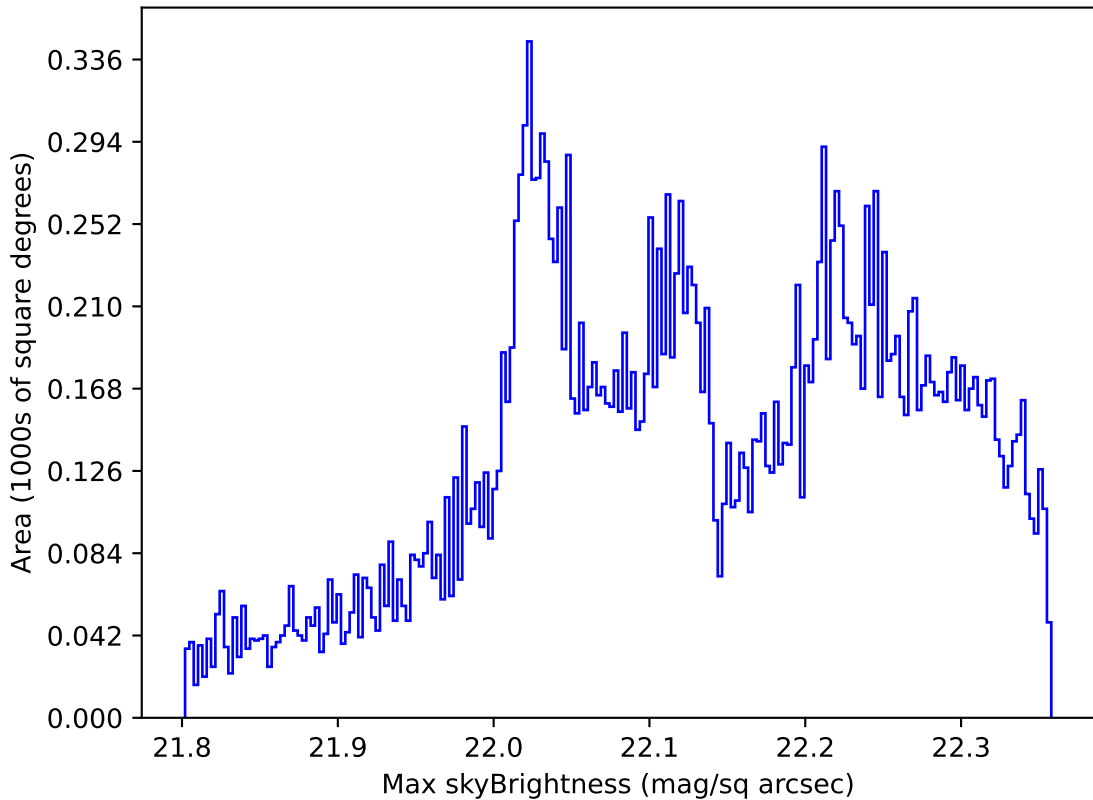
too_elab_2yr_r32_d2_ugrizy_v3.4_10yrs All sky g band: Max skyBrightness
