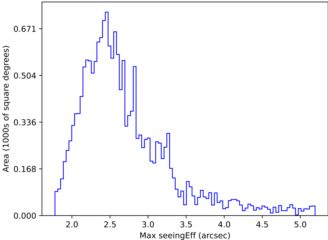
too_elab_2yr_r32_d2_ugrizy_v3.4_10yrs WFD i band: Max seeingEff
