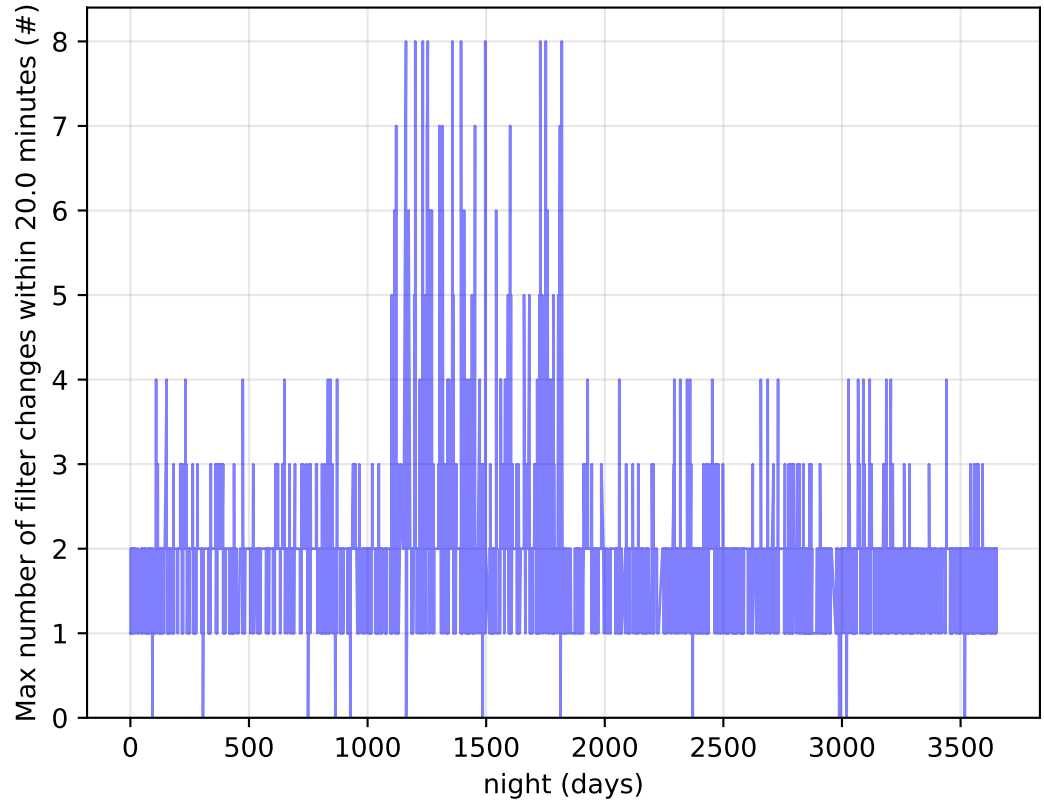
too_elab_2yr_r32_d2_ugrizy_v3.4_10yrs Per Night: Max number of filter changes within 20.0 minutes
