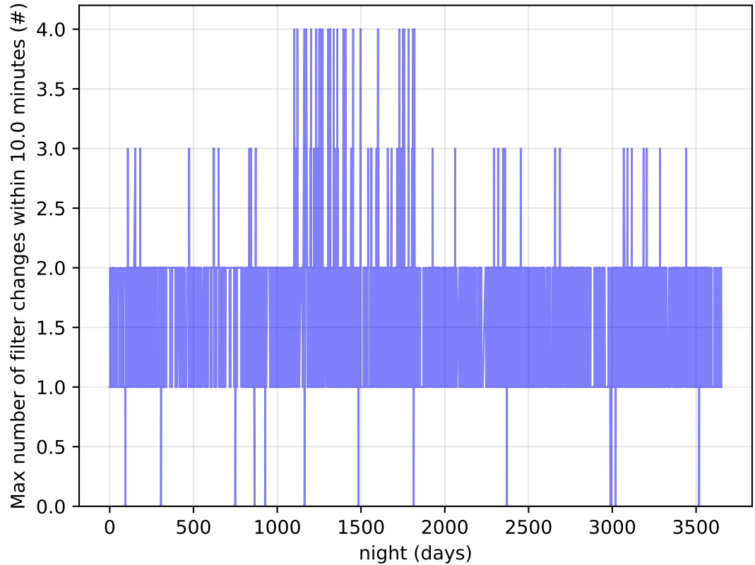
too_elab_2yr_r32_d2_ugrizy_v3.4_10yrs Per Night: Max number of filter changes within 10.0 minutes
