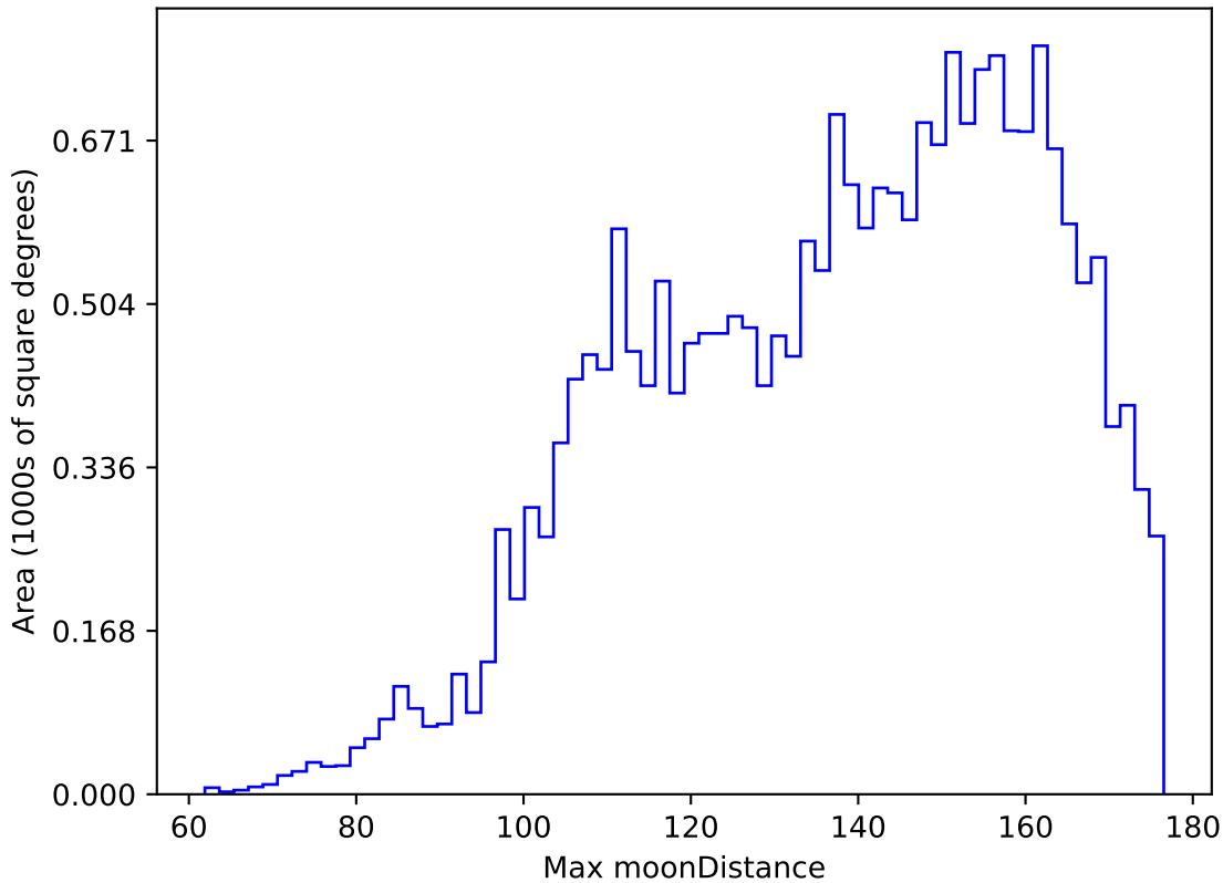
too_elab_2yr_r32_d2_ugrizy_v3.4_10yrs All sky y band: Max moonDistance
