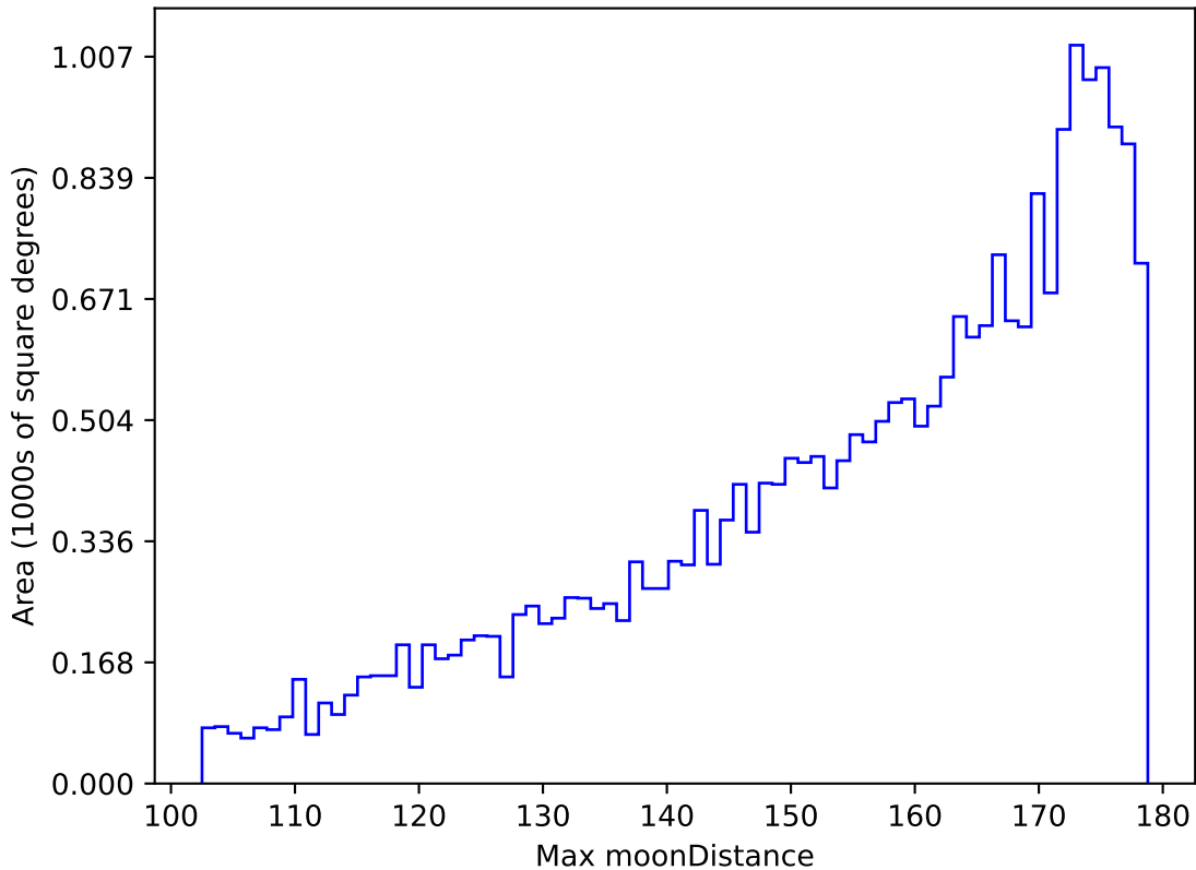
too_elab_2yr_r32_d2_ugrizy_v3.4_10yrs All sky g band: Max moonDistance
