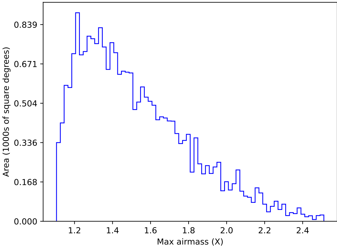
too_elab_2yr_r32_d2_ugrizy_v3.4_10yrs Yr 1 u band: Max airmass
