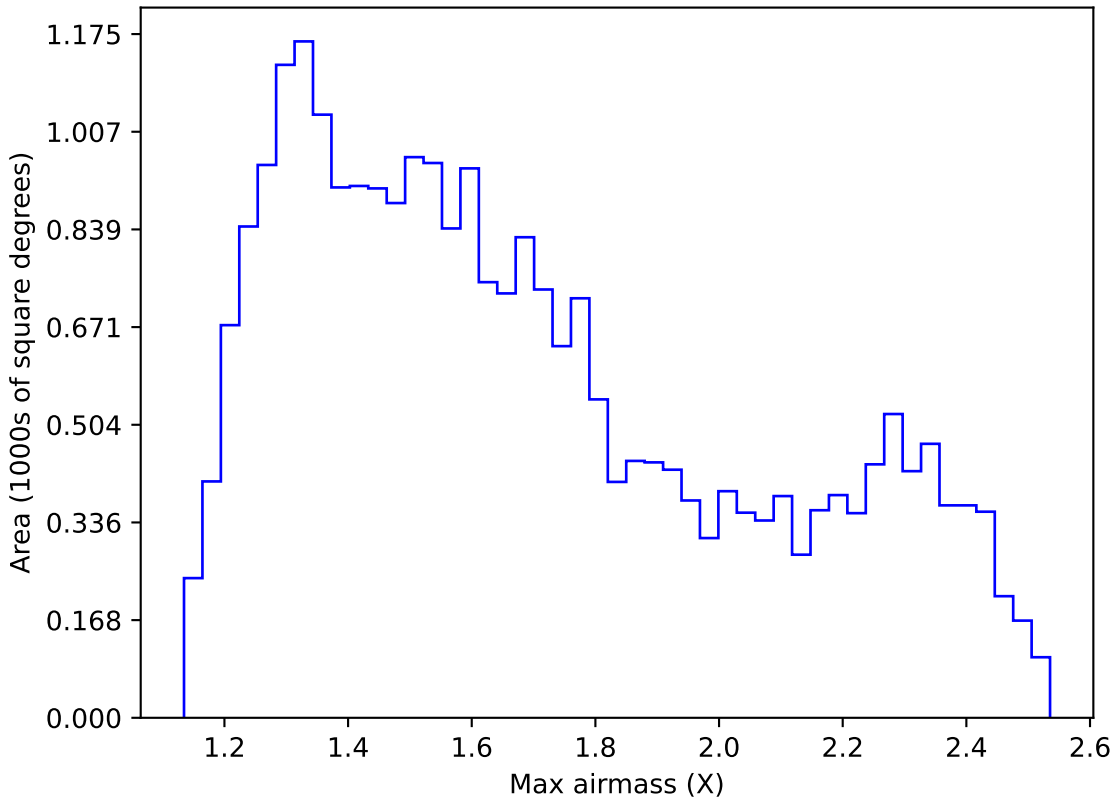
too_elab_2yr_r32_d2_ugrizy_v3.4_10yrs Yr 1 r band: Max airmass
