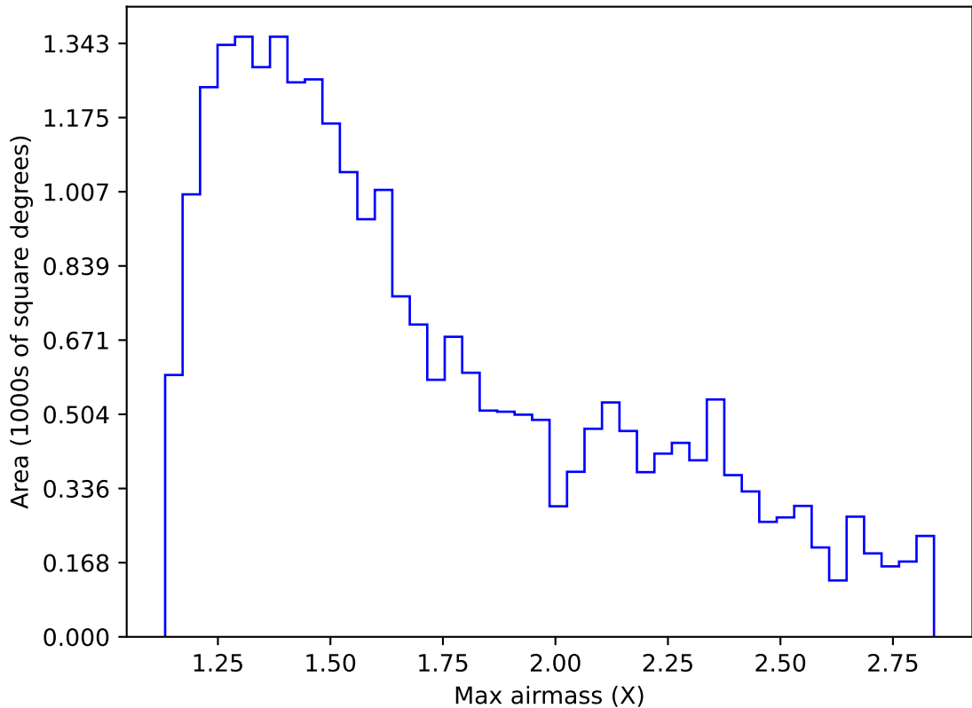
too_elab_2yr_r32_d2_ugrizy_v3.4_10yrs Yr 1 i band: Max airmass
