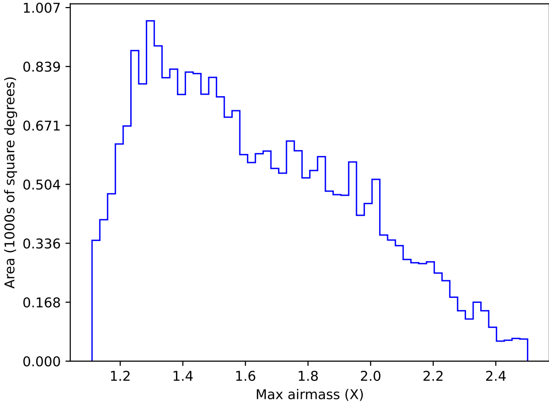
too_elab_2yr_r32_d2_ugrizy_v3.4_10yrs Yr 1 g band: Max airmass
